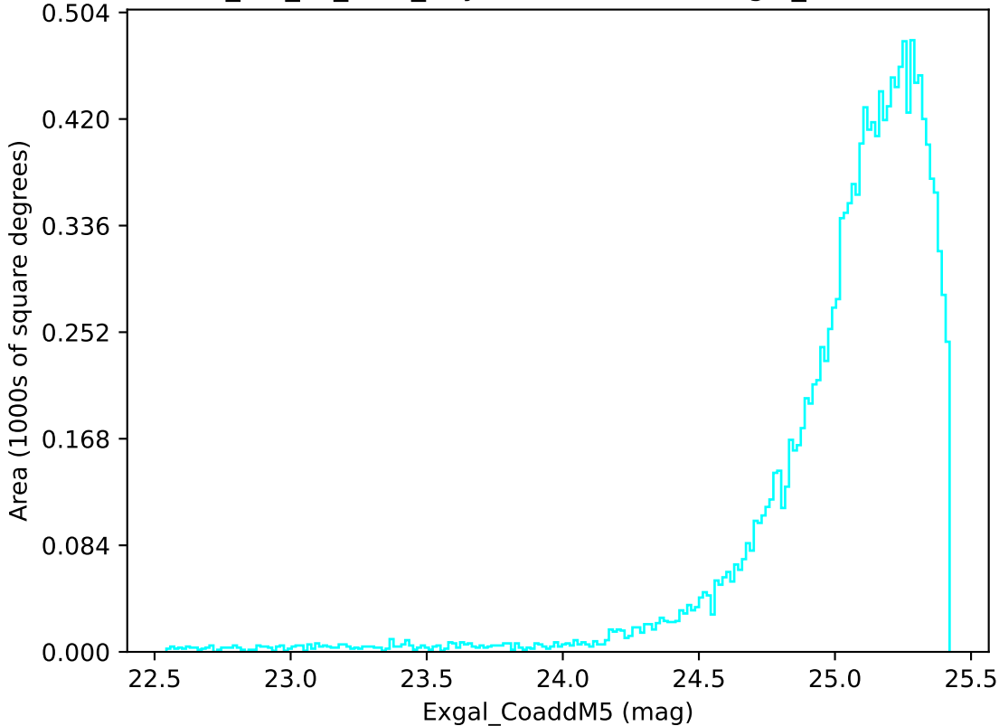
mw_roll_all_v3.3_10yrs WFD u band: Exgal_CoaddM5
