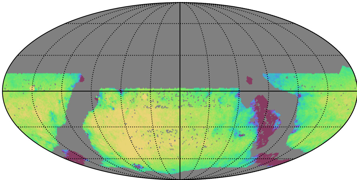
mw_roll_all_v3.3_10yrs WFD r band: Exgal_CoaddM5
