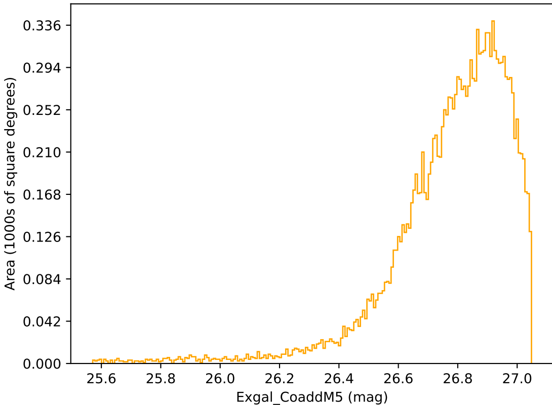
mw_roll_all_v3.3_10yrs WFD r band: Exgal_CoaddM5
