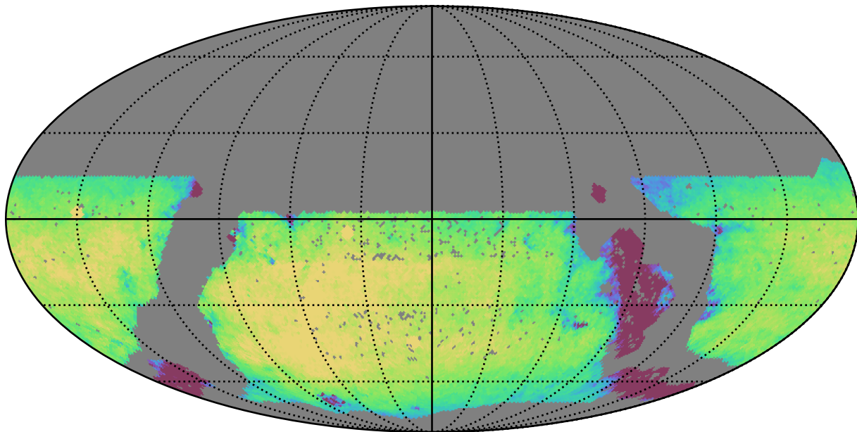
mw_roll_all_v3.3_10yrs WFD i band: Exgal_CoaddM5
