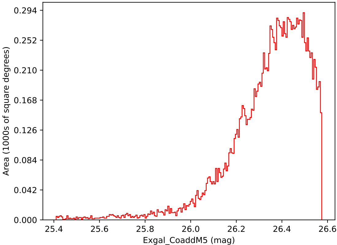
mw_roll_all_v3.3_10yrs WFD i band: Exgal_CoaddM5
