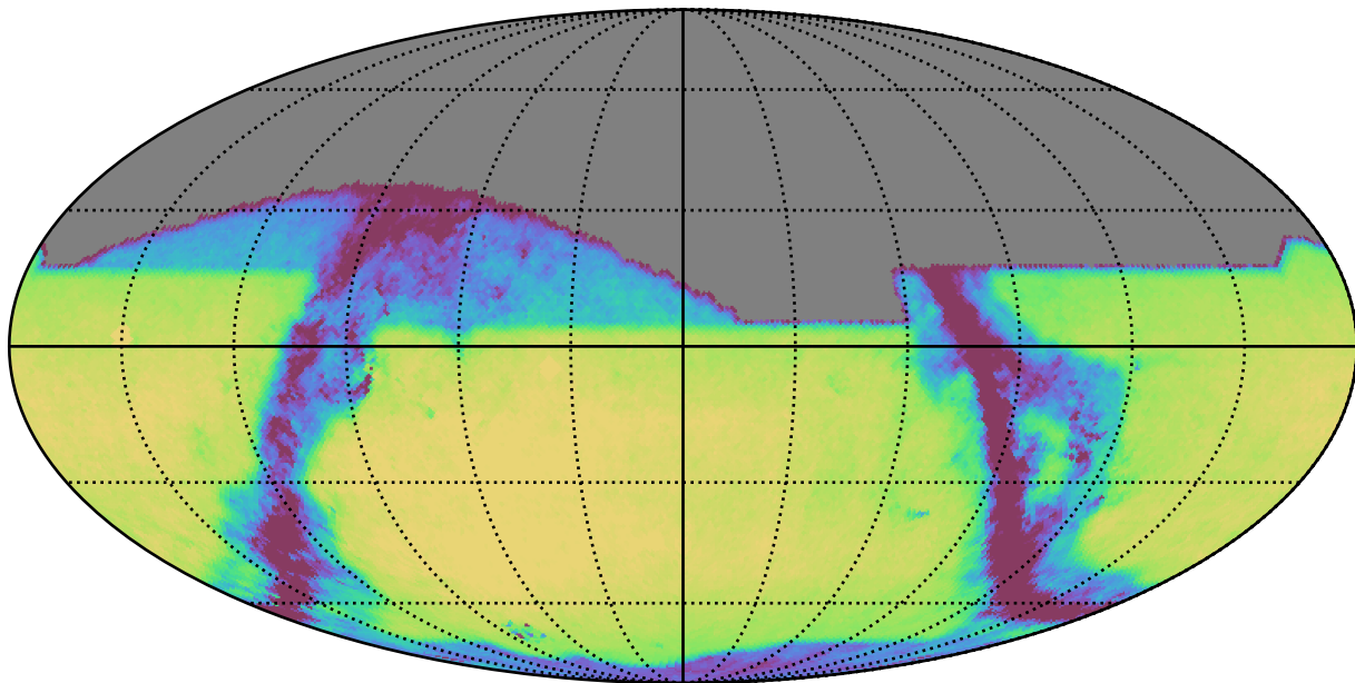
mw_roll_all_v3.3_10yrs All sky z band: Exgal_CoaddM5
