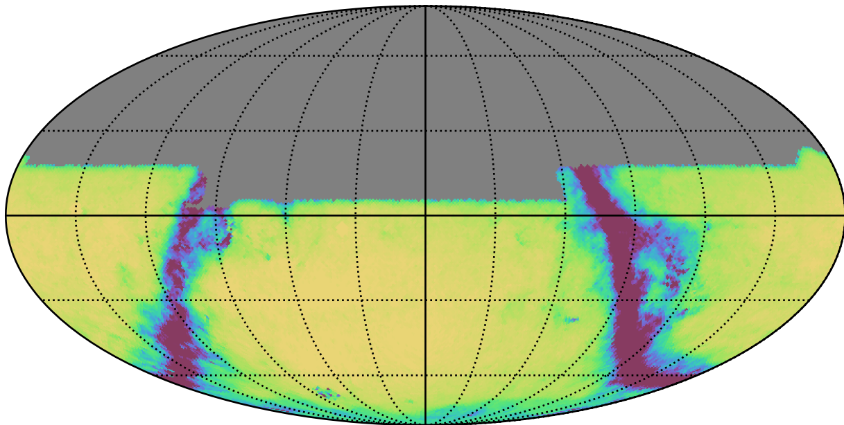
mw_roll_all_v3.3_10yrs All sky u band: Exgal_CoaddM5
