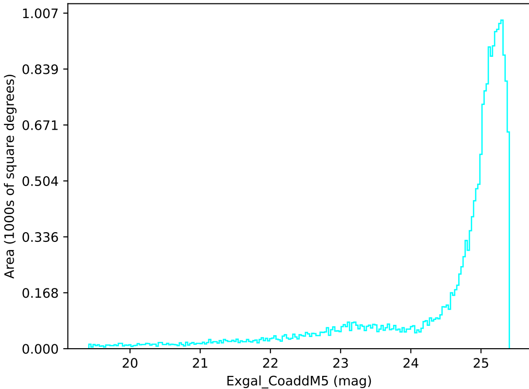
mw_roll_all_v3.3_10yrs All sky u band: Exgal_CoaddM5
