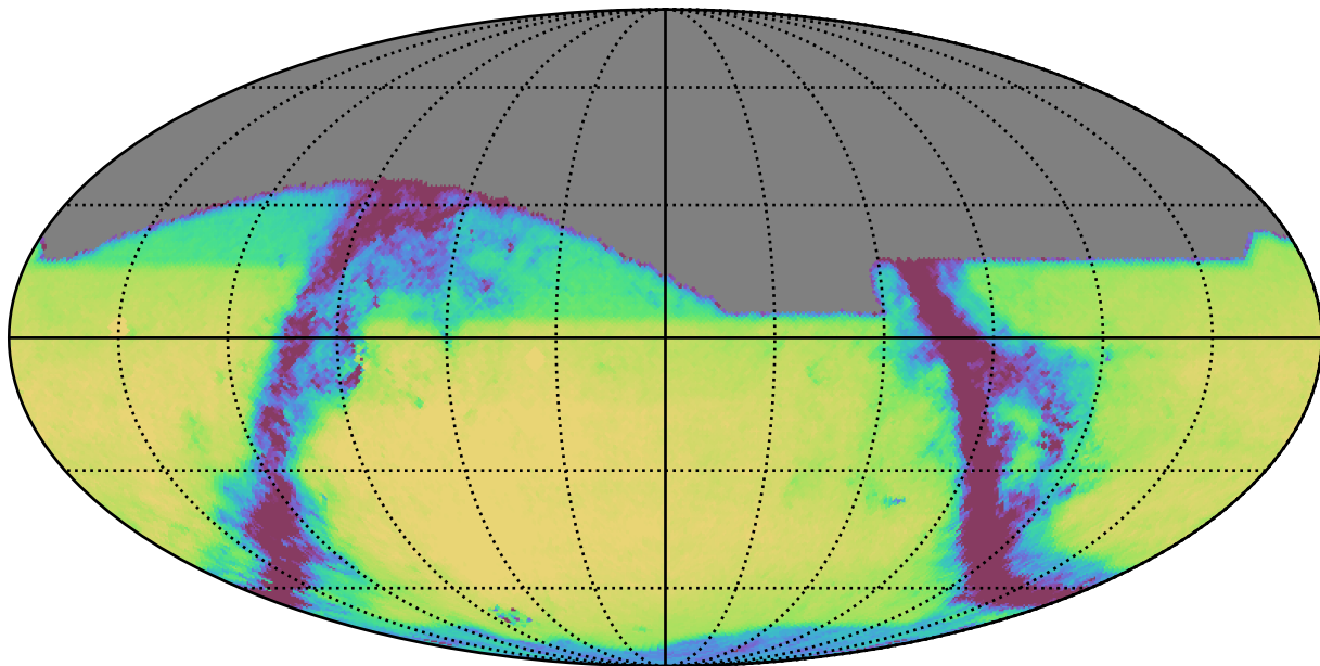
mw_roll_all_v3.3_10yrs All sky r band: Exgal_CoaddM5
