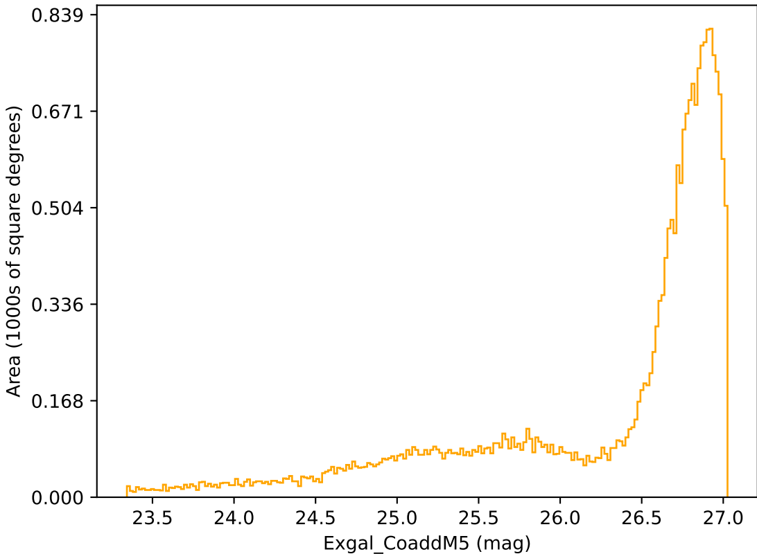
mw_roll_all_v3.3_10yrs All sky r band: Exgal_CoaddM5
