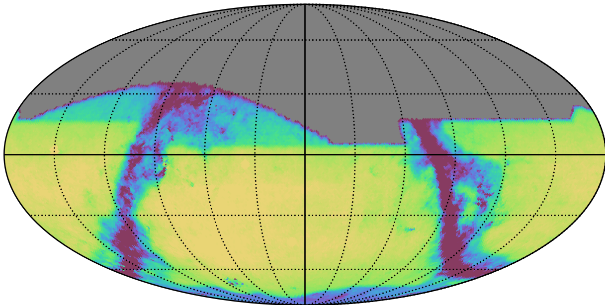
mw_roll_all_v3.3_10yrs All sky i band: Exgal_CoaddM5
