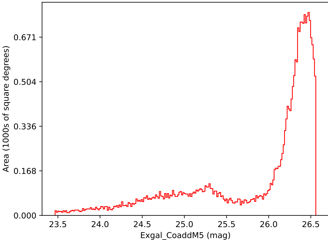
mw_roll_all_v3.3_10yrs All sky i band: Exgal_CoaddM5
