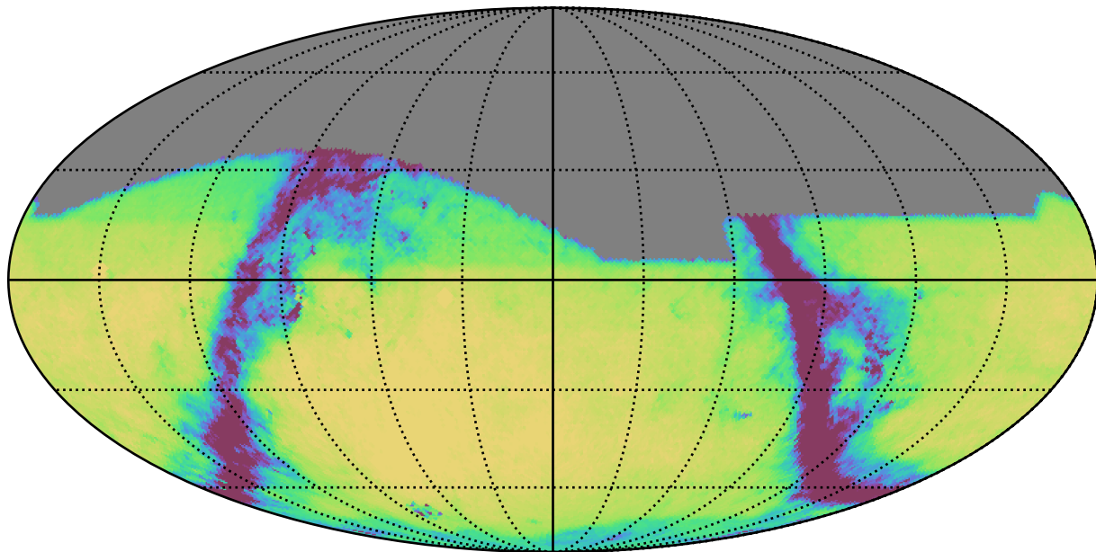
mw_roll_all_v3.3_10yrs All sky g band: Exgal_CoaddM5
