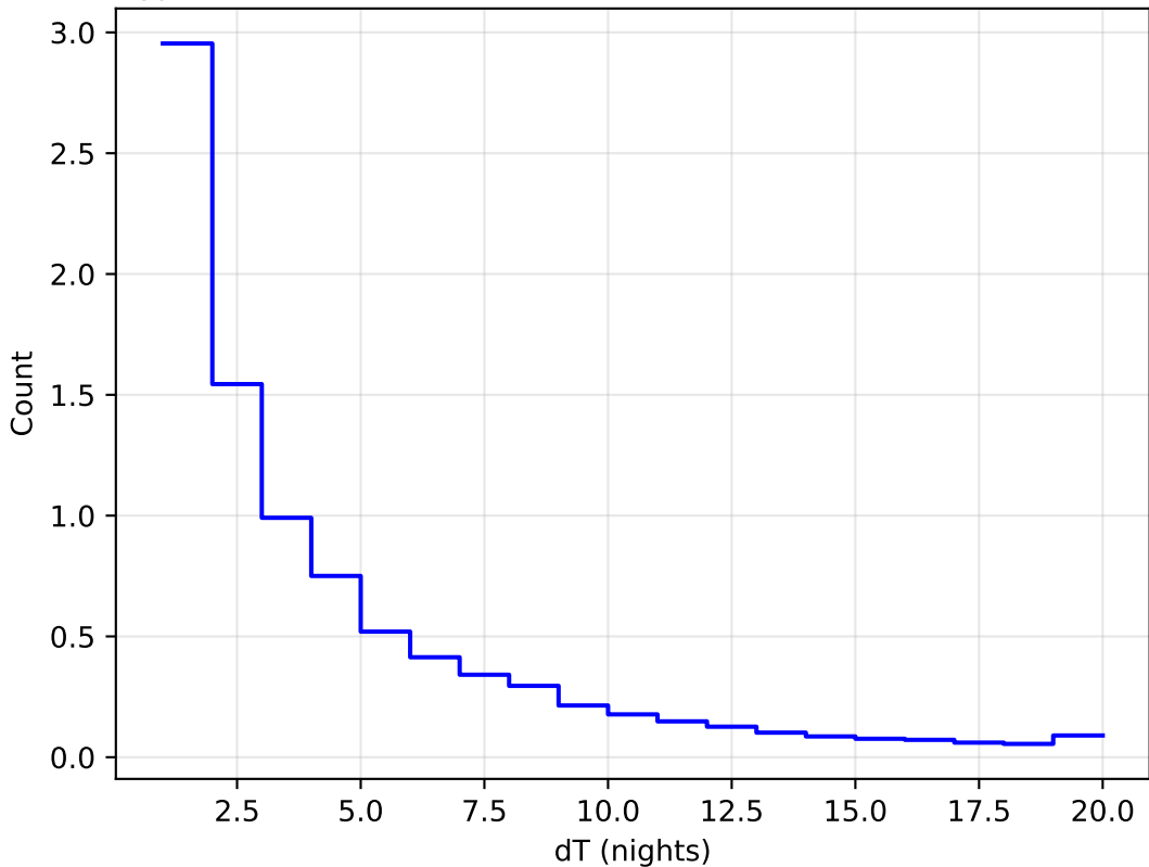
mw_roll_all_v3.3_10yrs All sky all bands: DeltaNight Histogram 1e6
