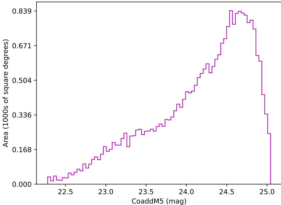
mw_roll_all_v3.3_10yrs Yr 3-4 z band: CoaddM5
