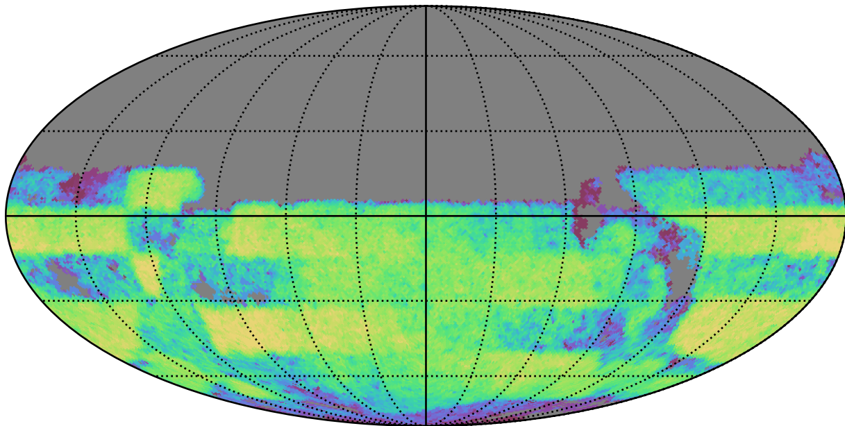
mw_roll_all_v3.3_10yrs Yr 3-4 y band: CoaddM5
