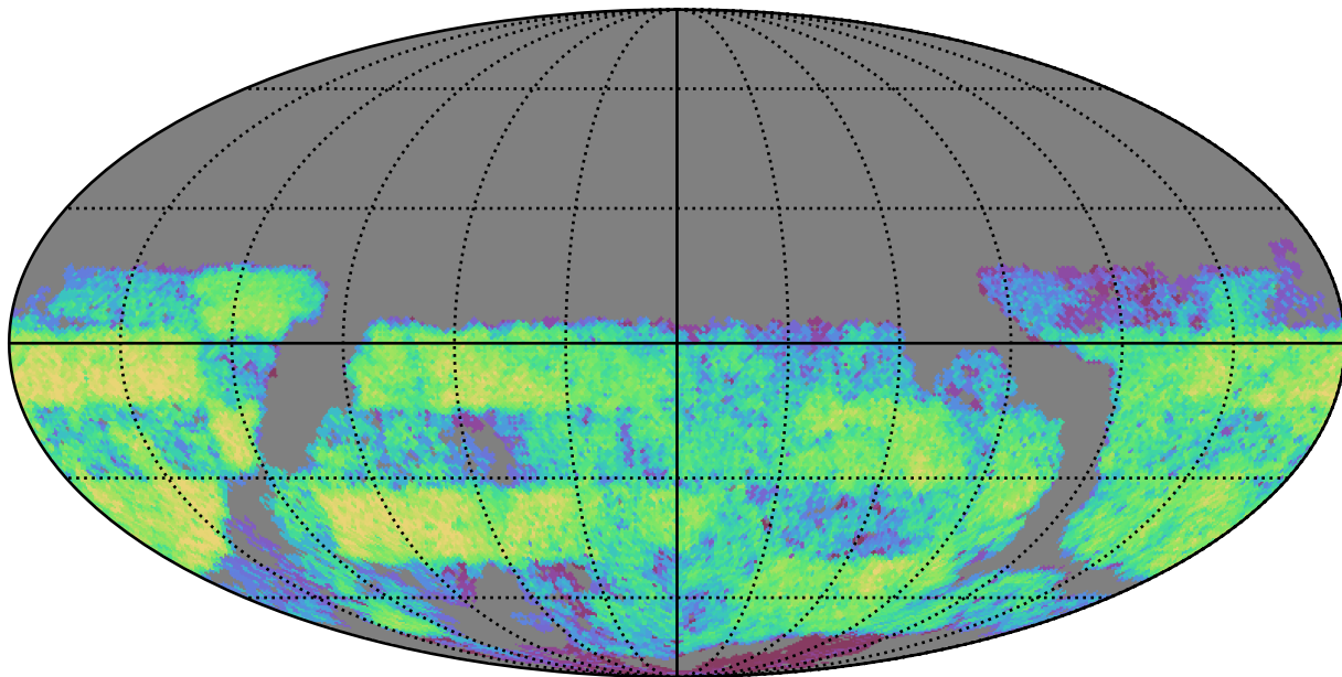
mw_roll_all_v3.3_10yrs Yr 3-4 u band: CoaddM5
