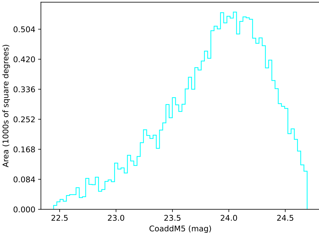
mw_roll_all_v3.3_10yrs Yr 3-4 u band: CoaddM5
