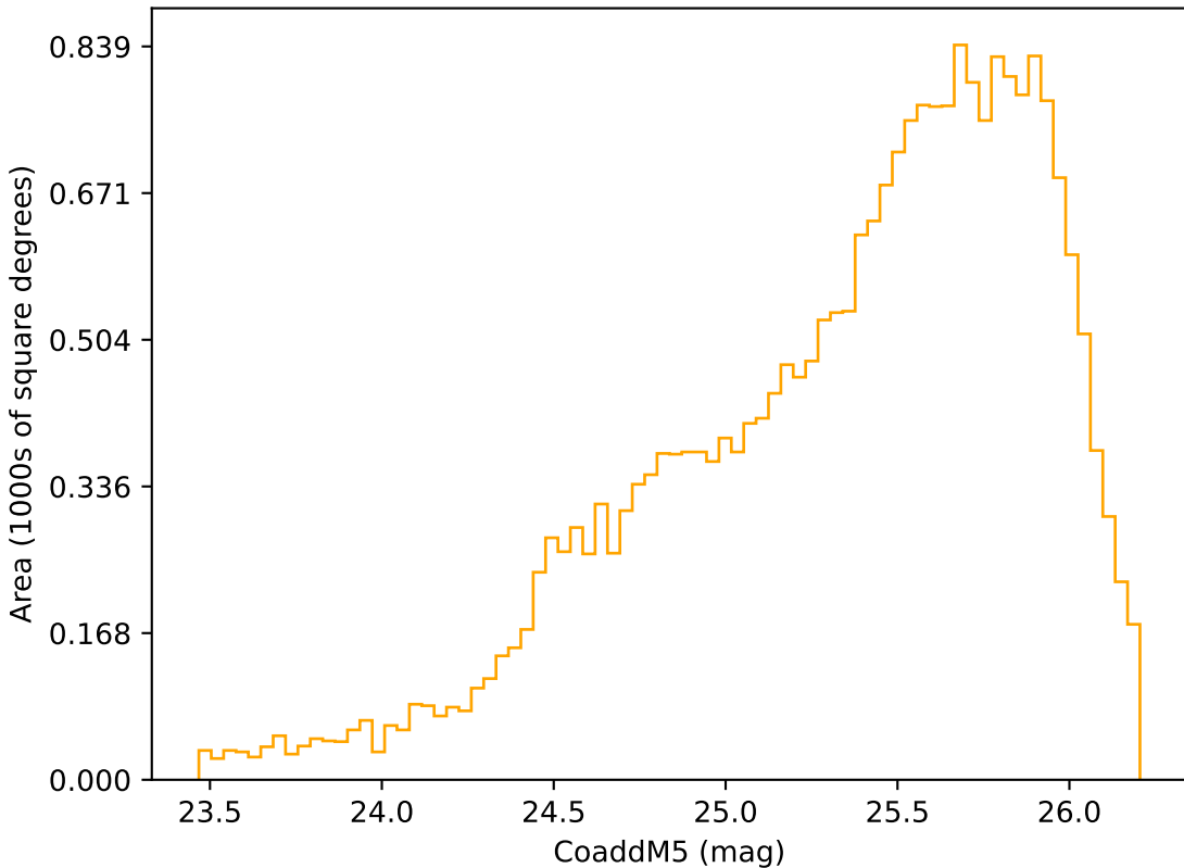
mw_roll_all_v3.3_10yrs Yr 3-4 r band: CoaddM5
