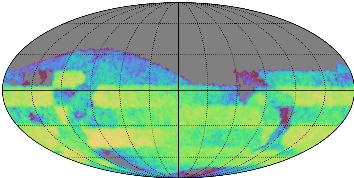
mw_roll_all_v3.3_10yrs Yr 3-4 i band: CoaddM5
