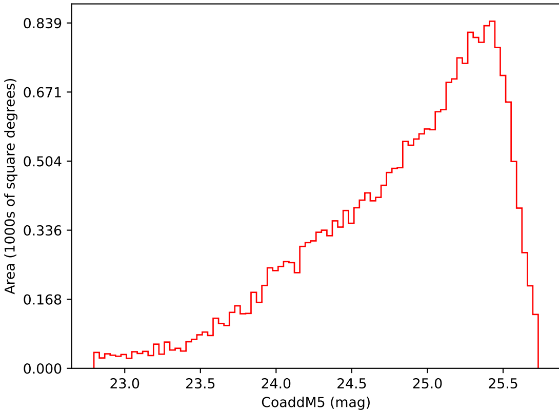
mw_roll_all_v3.3_10yrs Yr 3-4 i band: CoaddM5
