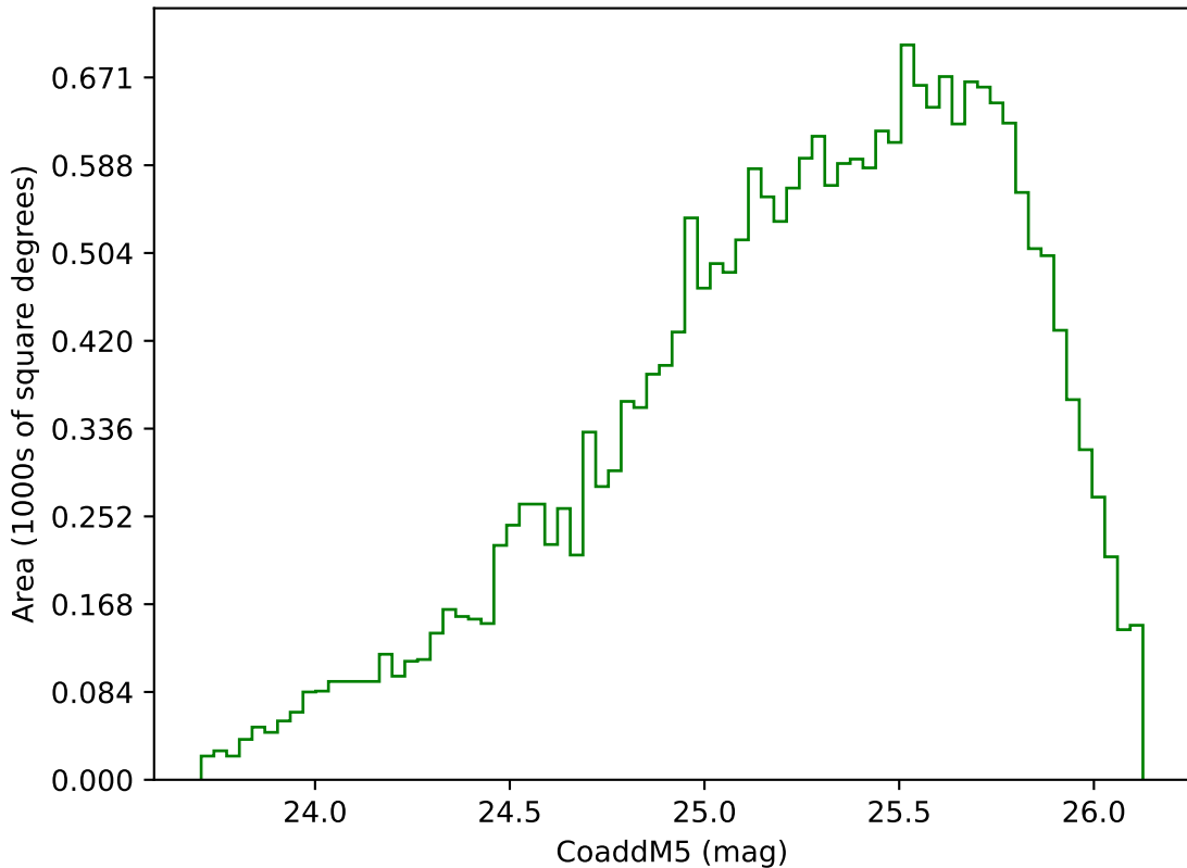
mw_roll_all_v3.3_10yrs Yr 3-4 g band: CoaddM5
