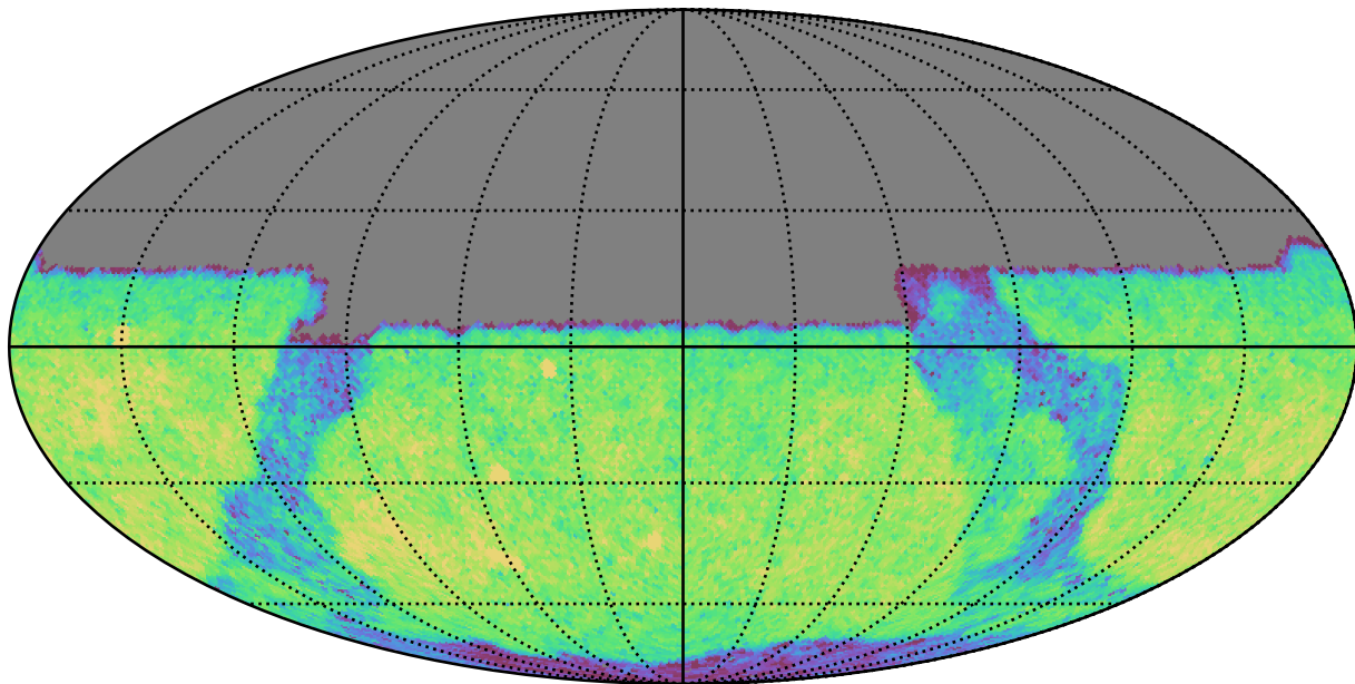
mw_roll_all_v3.3_10yrs Yr 1 y band: CoaddM5
