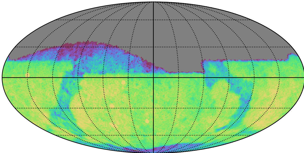
mw_roll_all_v3.3_10yrs Yr 1 r band: CoaddM5
