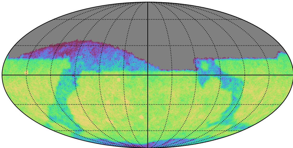
mw_roll_all_v3.3_10yrs Yr 1 i band: CoaddM5
