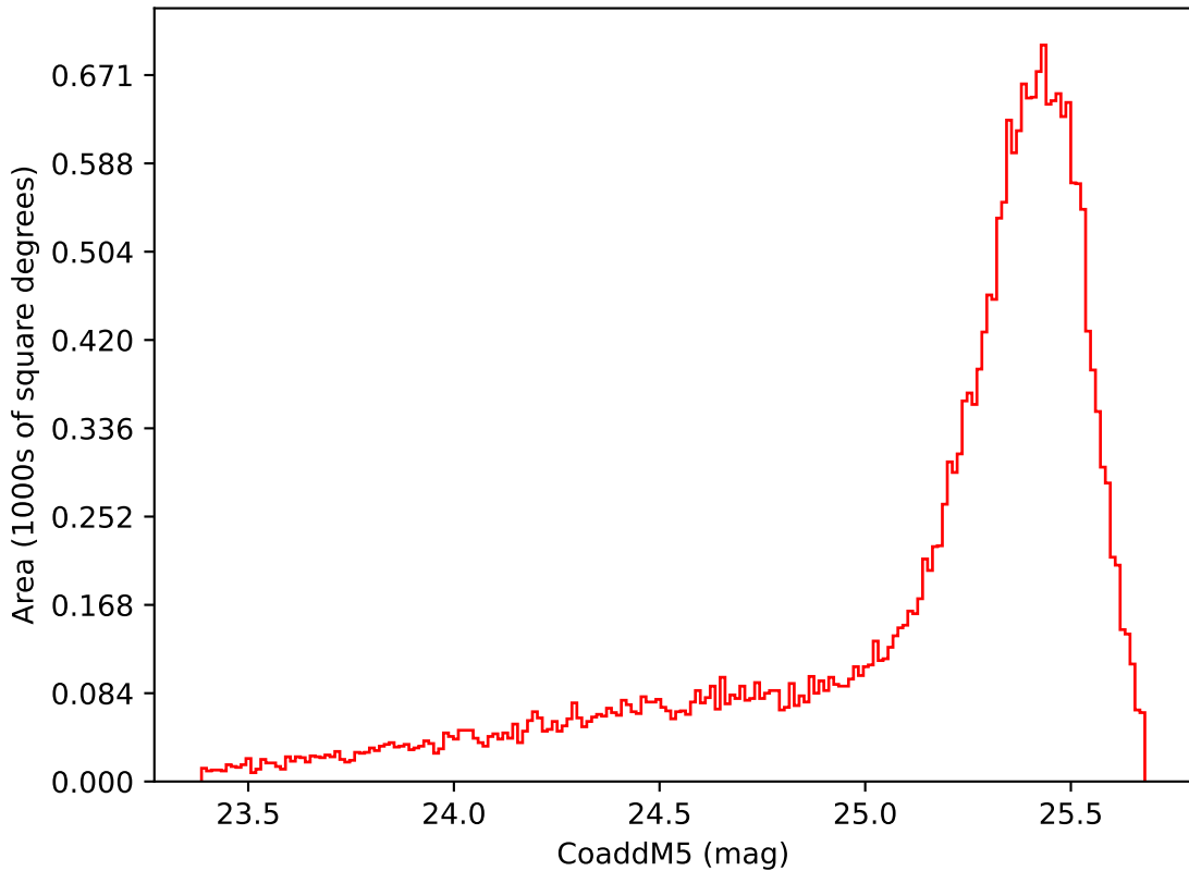
mw_roll_all_v3.3_10yrs Yr 1 i band: CoaddM5
