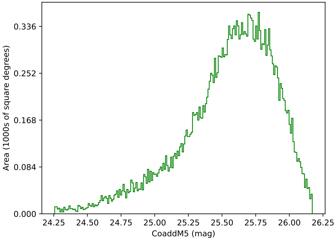
mw_roll_all_v3.3_10yrs Yr 1 g band: CoaddM5
