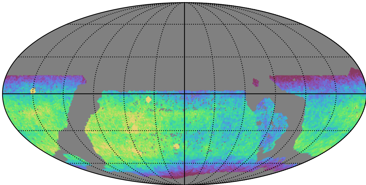
mw_roll_all_v3.3_10yrs WFD z band: CoaddM5
