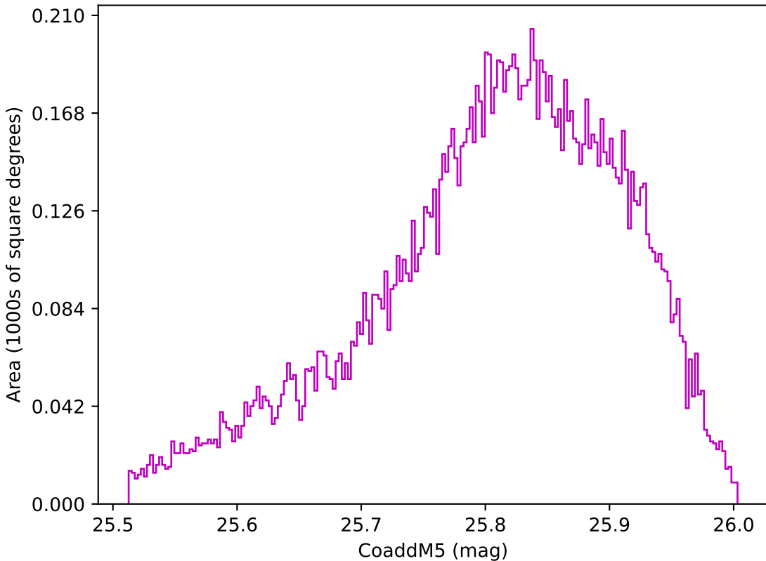
mw_roll_all_v3.3_10yrs WFD z band: CoaddM5
