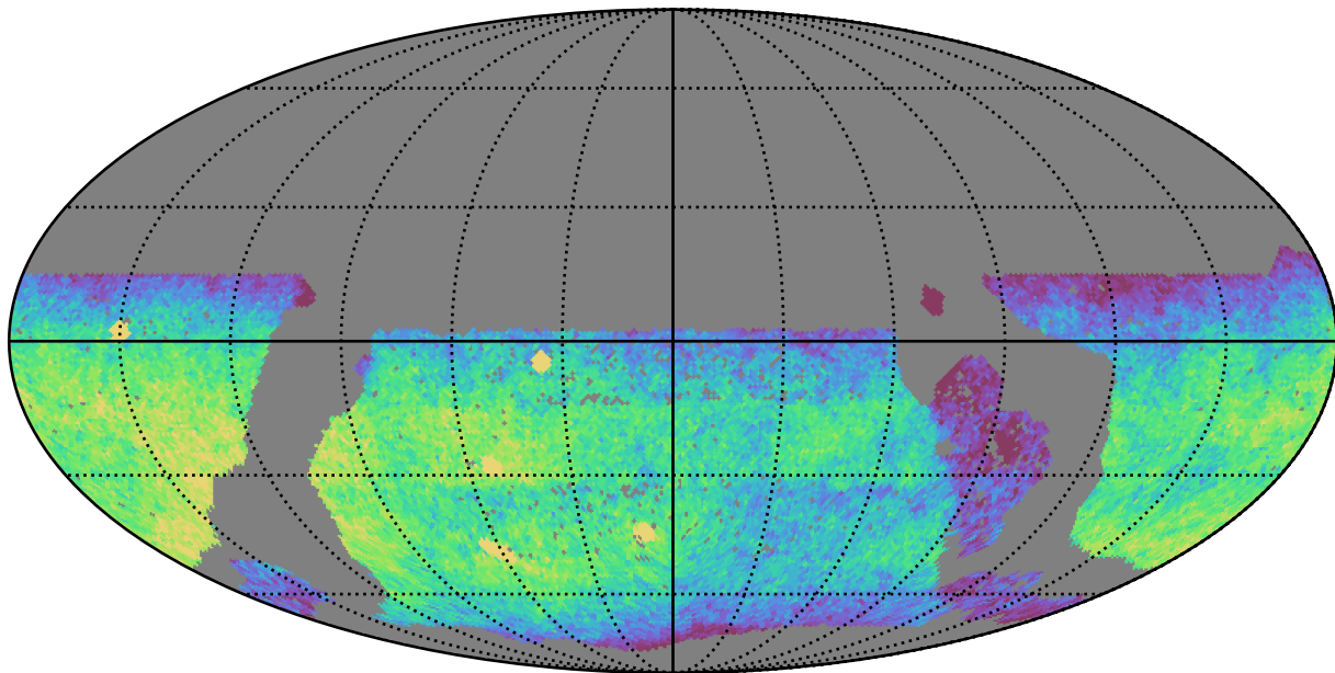
mw_roll_all_v3.3_10yrs WFD u band: CoaddM5
