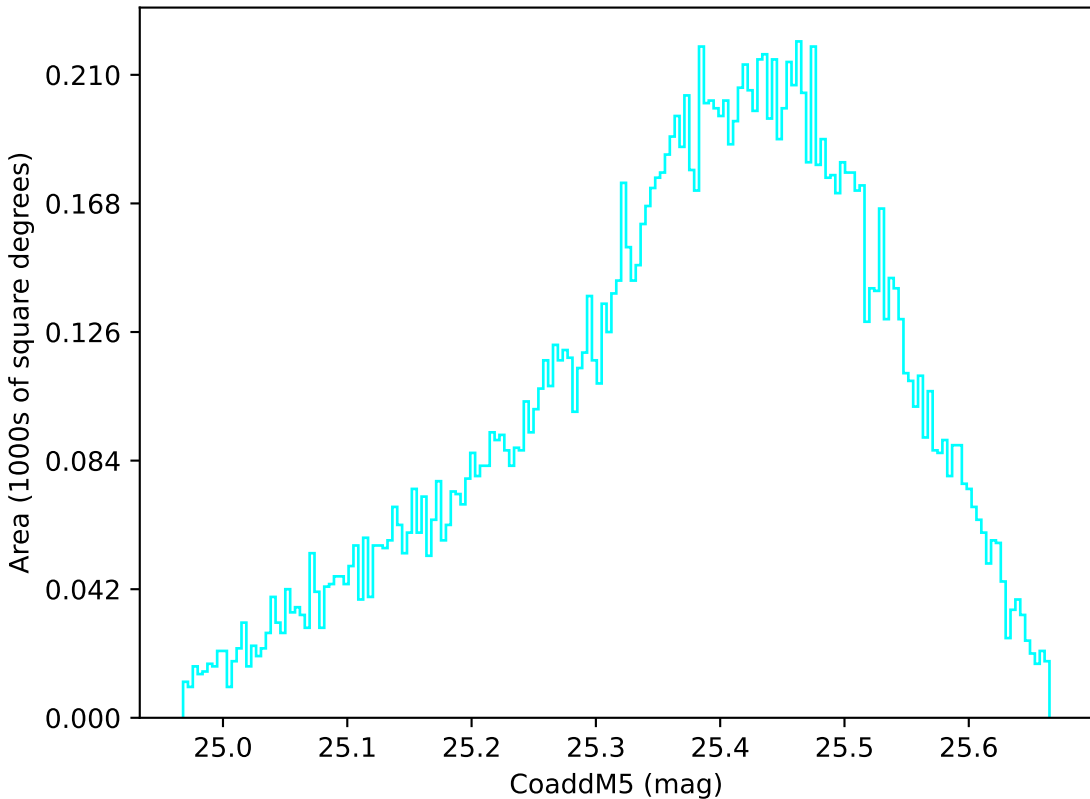
mw_roll_all_v3.3_10yrs WFD u band: CoaddM5
