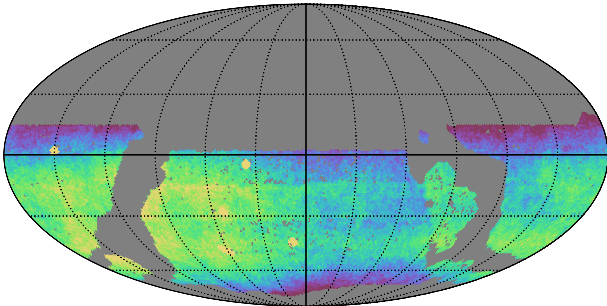
mw_roll_all_v3.3_10yrs WFD r band: CoaddM5
