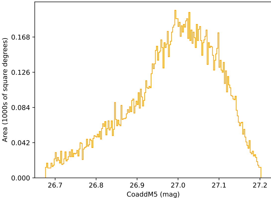
mw_roll_all_v3.3_10yrs WFD r band: CoaddM5
