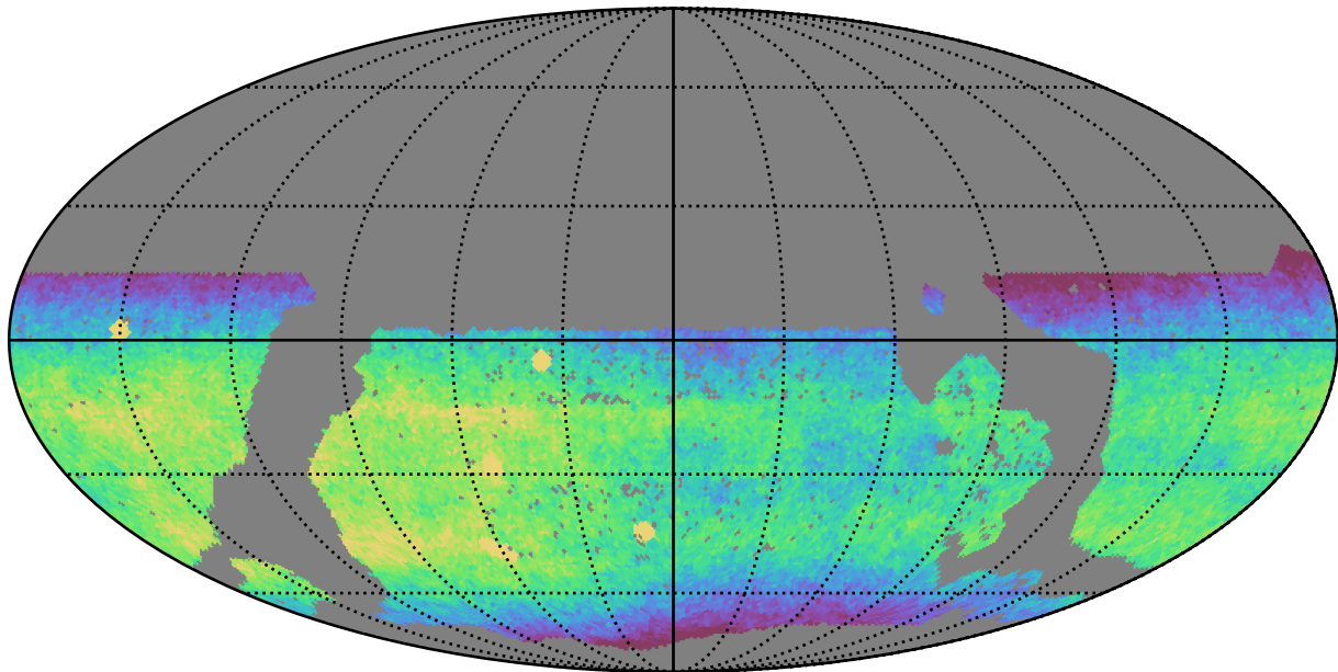
mw_roll_all_v3.3_10yrs WFD i band: CoaddM5
