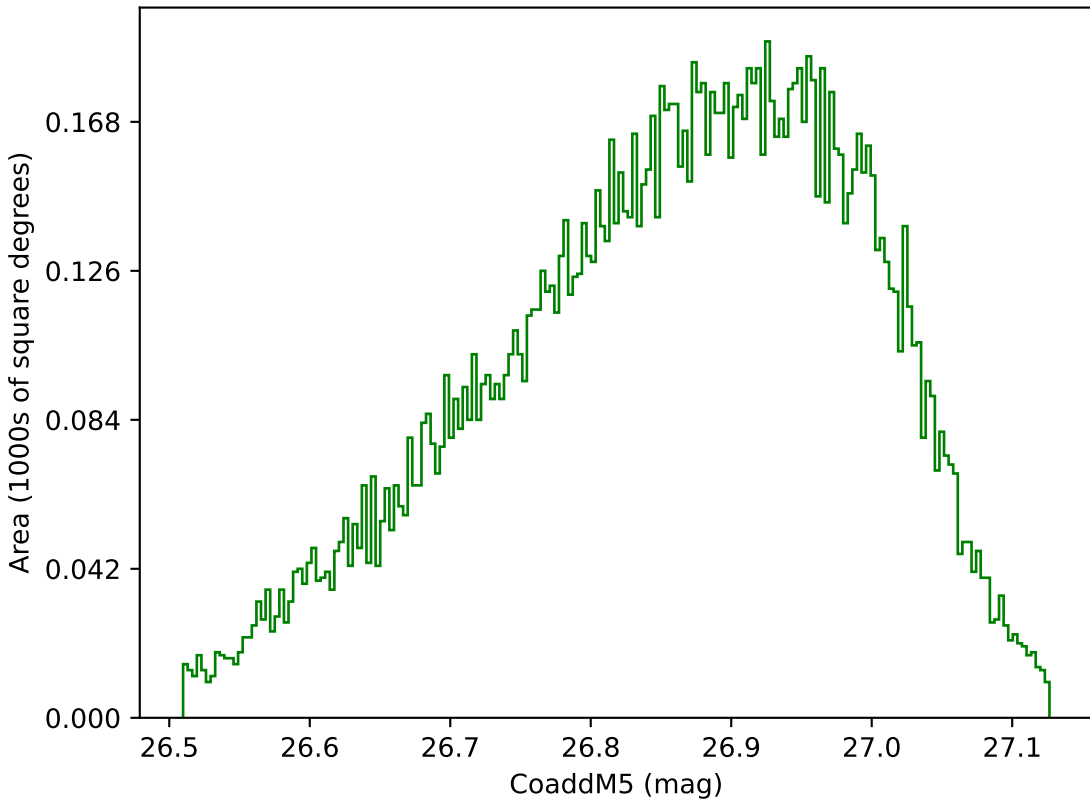
mw_roll_all_v3.3_10yrs WFD g band: CoaddM5
