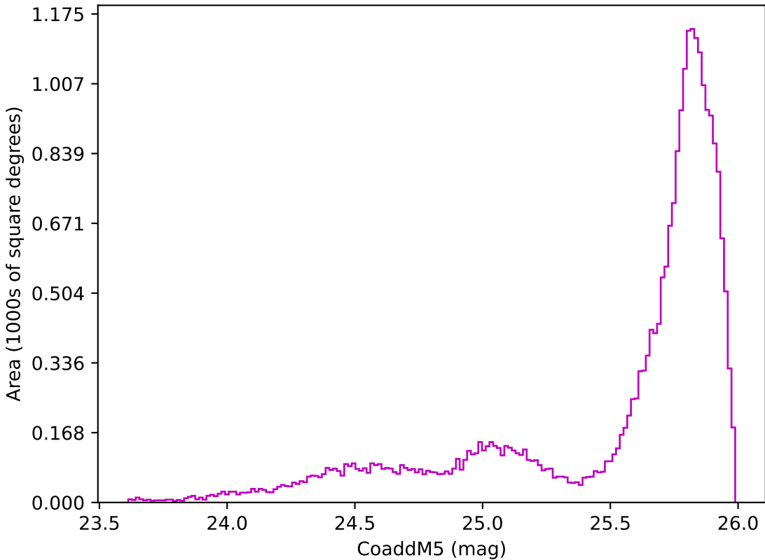
mw_roll_all_v3.3_10yrs All sky z band: CoaddM5
