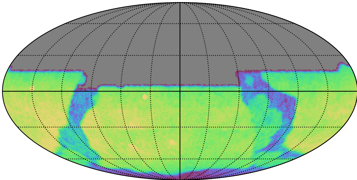
mw_roll_all_v3.3_10yrs All sky u band: CoaddM5
