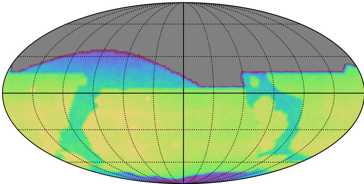
mw_roll_all_v3.3_10yrs All sky r band: CoaddM5
