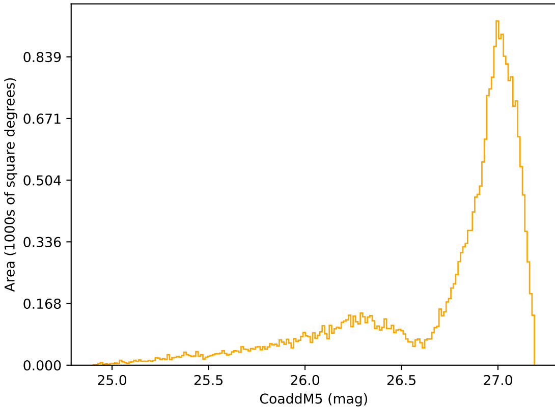
mw_roll_all_v3.3_10yrs All sky r band: CoaddM5
