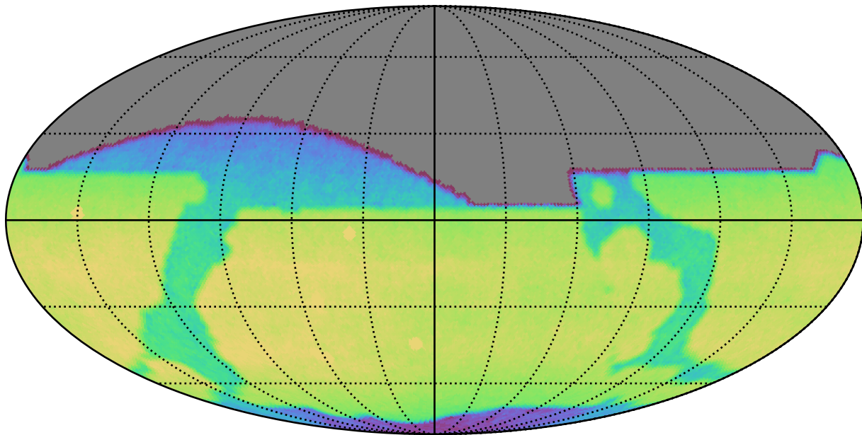
mw_roll_all_v3.3_10yrs All sky i band: CoaddM5
