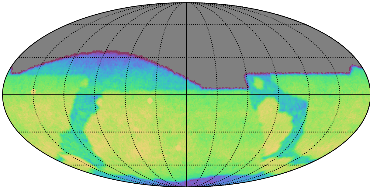
mw_roll_all_v3.3_10yrs All sky g band: CoaddM5
