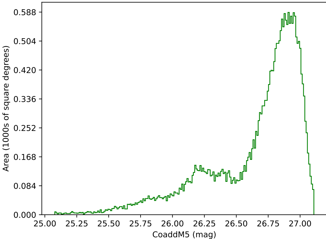
mw_roll_all_v3.3_10yrs All sky g band: CoaddM5
