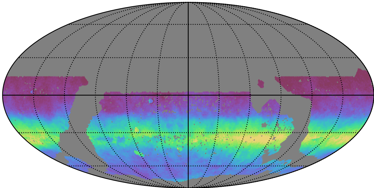
mw_roll_all_v3.3_10yrs WFD all bands: AngleRms rotSkyPos
