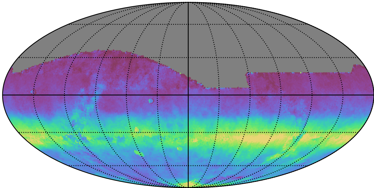
mw_roll_all_v3.3_10yrs All sky all bands: AngleRms rotSkyPos
