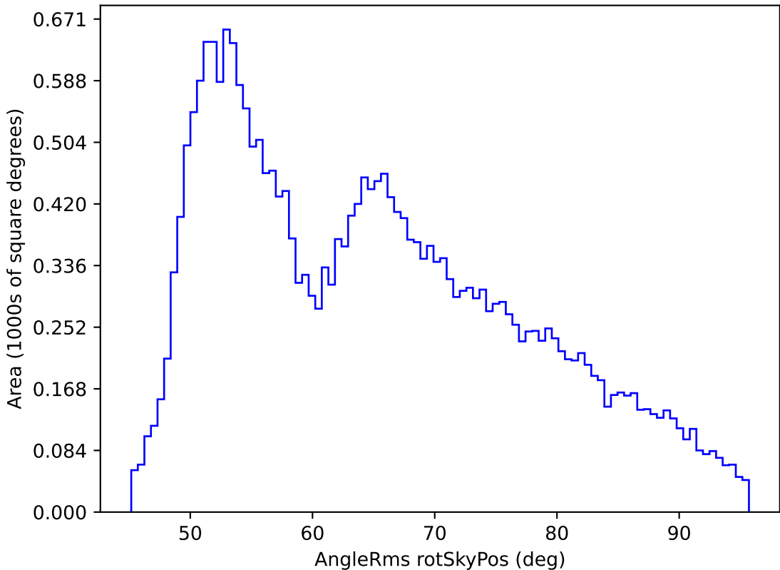
mw_roll_all_v3.3_10yrs All sky all bands: AngleRms rotSkyPos
