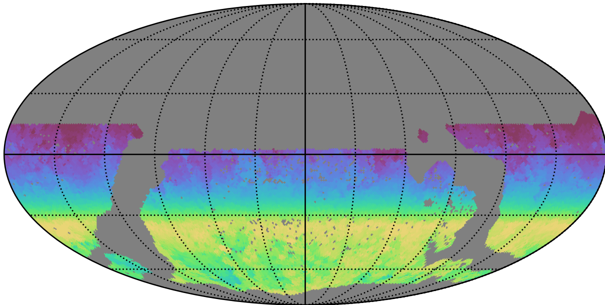
mw_roll_all_v3.3_10yrs WFD all bands: AngleRange rotSkyPos
