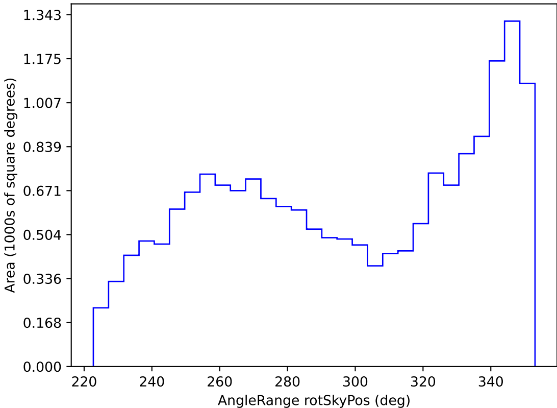
mw_roll_all_v3.3_10yrs WFD all bands: AngleRange rotSkyPos
