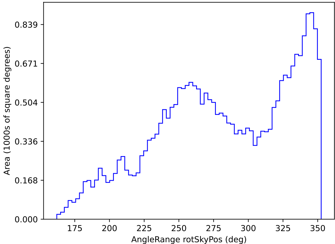
mw_roll_all_v3.3_10yrs All sky all bands: AngleRange rotSkyPos
