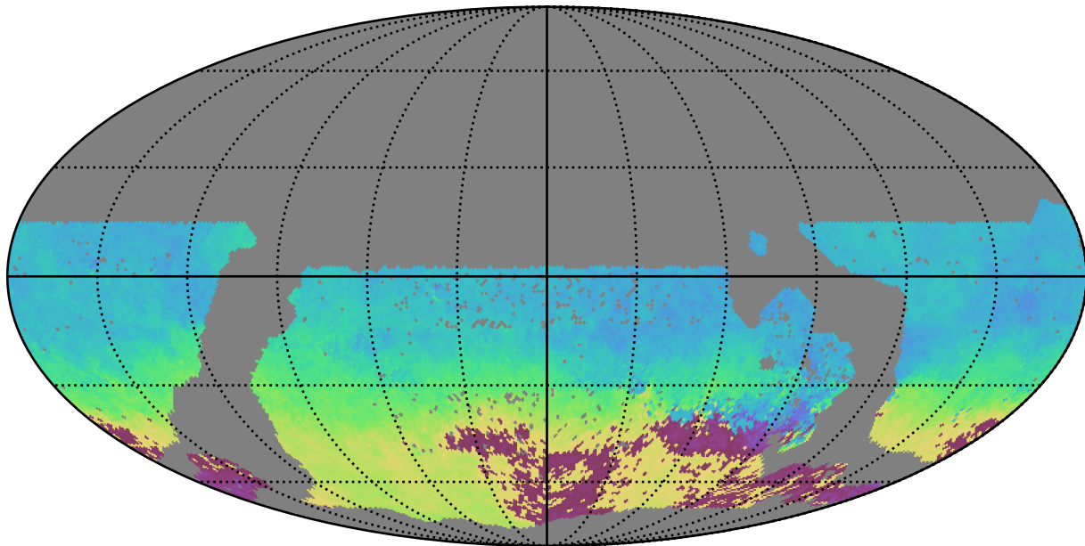
mw_roll_all_v3.3_10yrs WFD u band: AngleMean rotSkyPos
