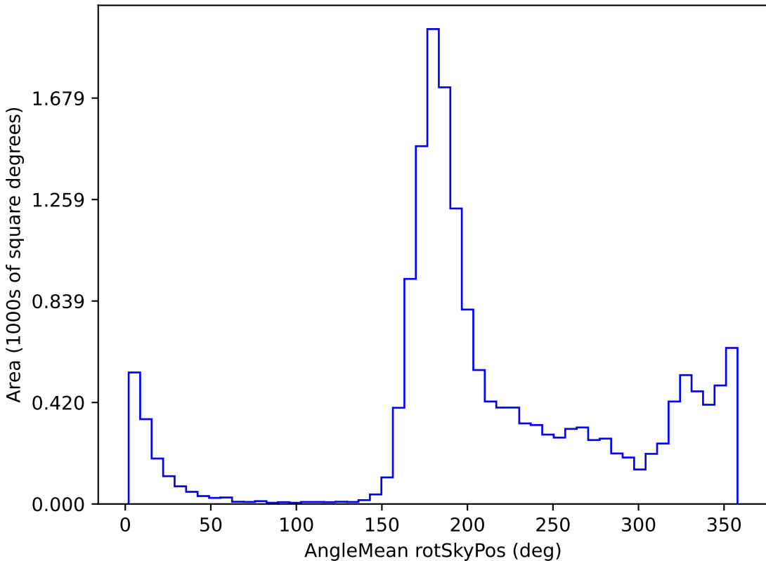
mw_roll_all_v3.3_10yrs WFD u band: AngleMean rotSkyPos
